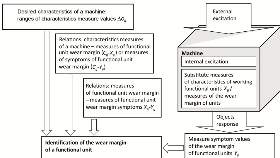
Fig. 4. The algorithm for the identification of the wear margin of a functional unit of a working object [4].
